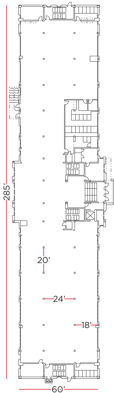
1st Floor
